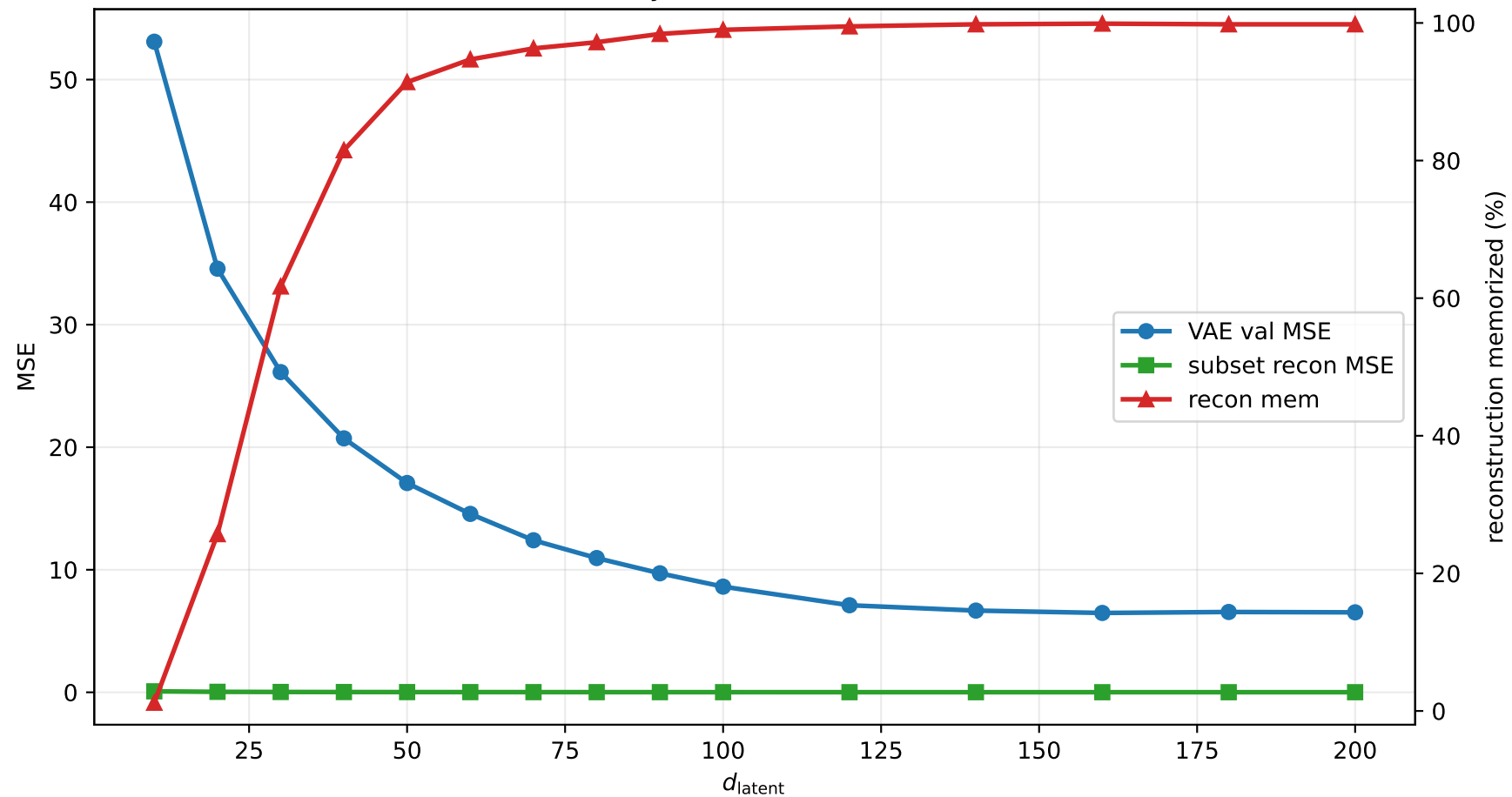
CelebA: VAE Quality vs Reconstruction Memorization
